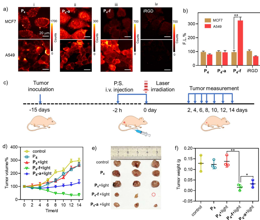
Fig. 8 (a) Fluorescence images of A549 and MCF7 cells after incubation with P_4 (8 \mu\text{M} , group i), P_4 -a (8 \mu\text{M} , group ii), or P_4 -f (8 \mu\text{M} , group iii) for 30 min. For group iv, the cells were incubated with iRGD (20 \mu\text{M} ) for 1 h, then incubated with P_4 -f (8 \mu\text{M} ) for 30 min. \lambda_{\text{ex}} = 405 \text{ nm} ; \lambda_{\text{em}} = 647 \text{ nm} longpass filter. (b) Quantitative fluorescence intensity analysis of fluorescence images of i–iv in (a). Red: A549 brown: MCF7. (* P < 0.05 ; ** P < 0.01 ). The fluorescence of each compound in groups i–iv in MCF7 was calculated as 100%, and the fluorescence intensity in A549 was expressed as a percentage of that in MCF7. (c) Schematic illustration of the treatment regimen. (d) Tumor volume variation curves for the mice in the “control (PBS)”, “ P_4 ”, “ P_4 + light”, “ P_4 -f + light”, and “ P_4 -a + light” groups during the treatment period ( n = 3 , mean \pm SD). (e) Photographs of the tumours dissected from the mice in different groups. (f) Tumor weights of the mice in different groups at the end of treatment ( n = 3 , mean \pm SD).
