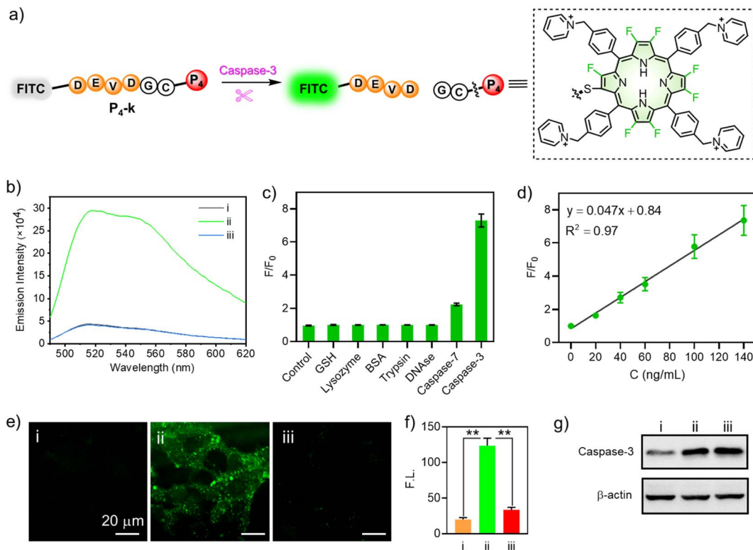
Fig. 7 (a) Schematic illustration of P_4 -k as a fluorescent sensor for caspase-3. (b) Fluorescence spectra of P_4 -k (10 \mu M) in PBS (pH 7.4) with selected treatments. P_4 -k alone for i; caspase-3 + P_4 -k for ii; inhibitor + caspase-3 + P_4 -k for iii at 37 ^{\circ} C for 1 h. \lambda_{\text{ex}} = 470 nm. (c) Fluorescence ratio ( F/F_0 ) response of P_4 -k to various species before ( F_0 ) and after ( F ) incubation with various species for 1 h in PBS (1 \times , pH 7.4). The concentration of GSH is 10 mM. The concentrations of lysozyme, BSA, trypsin, and DNase are all 1 \mu g mL ^{-1} . The concentrations of caspase-7 and caspase-3 are 200 ng mL ^{-1} . (d) Linear fitting curve of F/F_0 to the concentration of caspase-3 (0–140 ng mL ^{-1} ). \lambda_{\text{ex}} = 470 nm. The reaction was conducted in PBS (1 \times , pH 7.4) at 37 ^{\circ} C for 1 h. (e) Fluorescence microscope images. \lambda_{\text{ex}} = 488 nm; \lambda_{\text{em}} = 525/50 nm bandpass filter. Scale bar: 20 \mu m. (f) Quantitative fluorescence intensity analysis of cell images in (e). (g) Expression level of caspase-3 of HeLa cells measured by Western blot assay. (i): HeLa cells were treated with P_4 -k (10 \mu M) for 1 h. (ii): HeLa cells underwent induced apoptosis by STS (3 \mu M) for 2 h, and were then cultured with P_4 -k (10 \mu M) for 1 h. (iii): HeLa cells were successively cultured with caspase-3 (10 \mu M) inhibitor and STS (3 \mu M) for 2 h, then with P_4 -k (3 \mu M) for 1 h. (* P < 0.05 ; ** P < 0.01 ).
