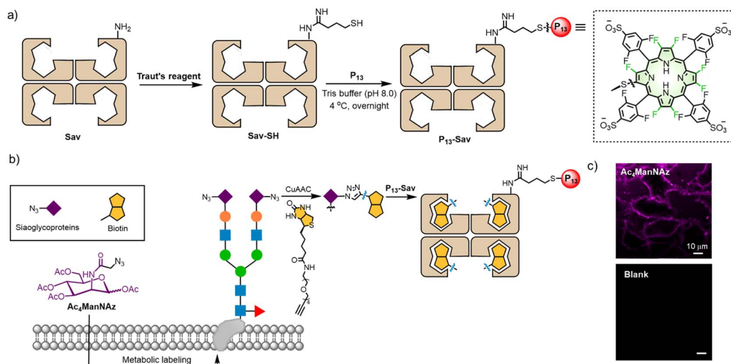
Fig. 6 Schematic illustration of (a) the synthesis of P 13 -Sav. (b) Ac 4 ManNAz metabolic labeling. (c) Fluorescence images of sialoglycoproteins using P 13 -Sav. \lambda_{\text{ex}} = 405 \text{ nm} ; \lambda_{\text{em}} = 647 \text{ nm} longpass filter. Scale bar: 10 \mu\text{m} .
