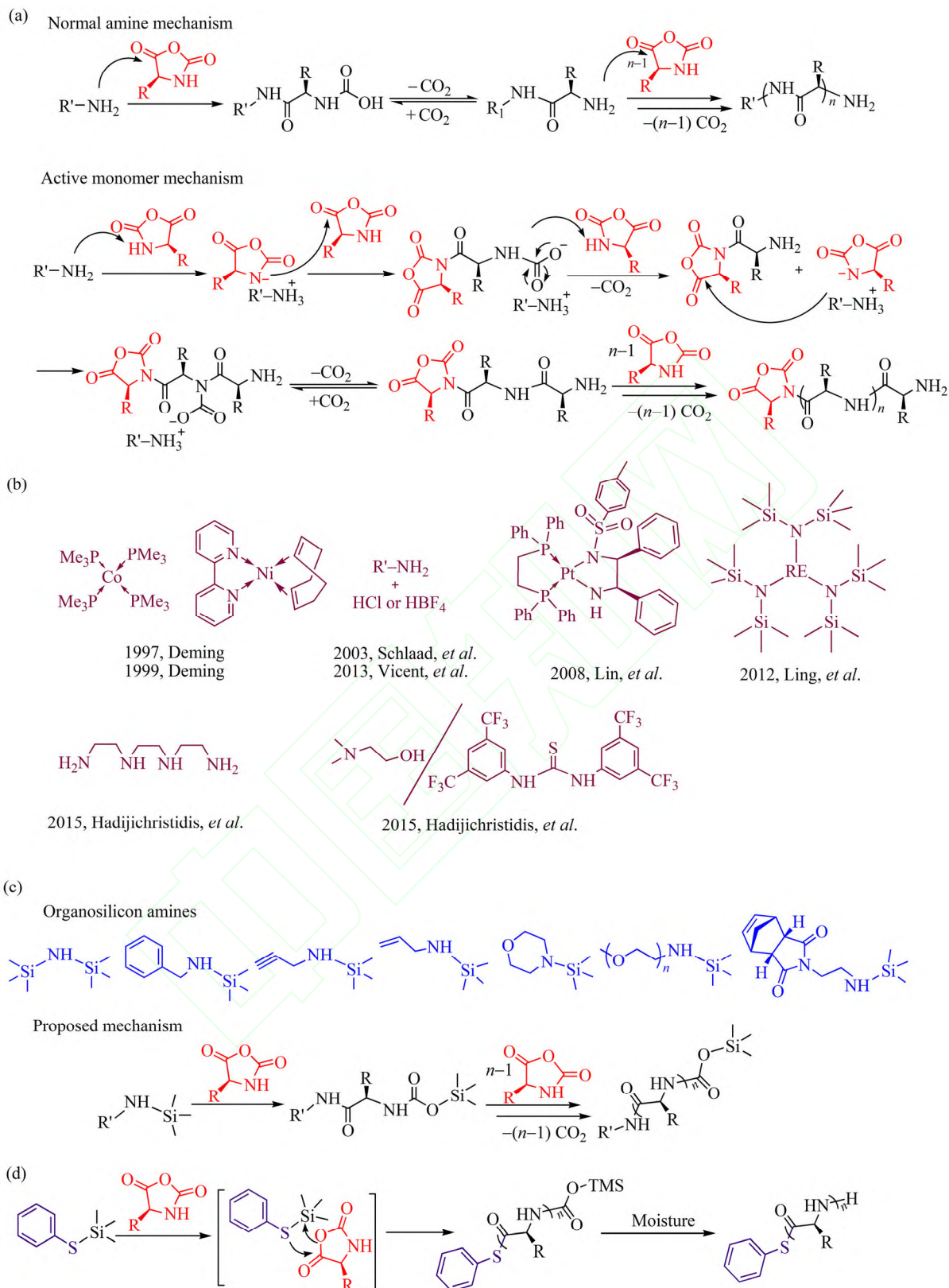
Fig. 1 (a) Two general ring-opening polymerization (ROP) mechanisms of \alpha -amino acid NCAs; (b) Examples of reported initiation systems successfully used in controlled ROP of NCAs; (c) Structures of organosilicon amines and proposed mechanisms; (d) PhS-TMS mediated NCA polymerization (Adapted with permission from Ref.[41]; Copyright (2016) American Chemical Society)
