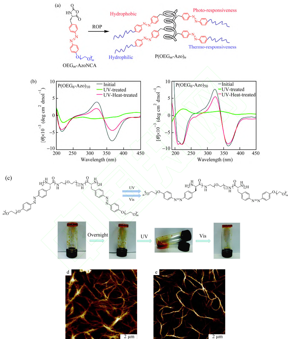
Fig. 4 (a) Synthesis of dual photo- and thermal- responsive P \alpha AAs; (b) CD spectra of \text{P(OEG}_6\text{-Azo)}_{10} and \text{P(OEG}_6\text{-Azo)}_{50} in 2,2,2-trifluoroethyl alcohol (the polymers were first irradiated with UV at 365 nm for 5 min, followed by heating at 70 °C for 60 min) (The online version is colorful.); (c) Photographs of triblock copolymer \text{P(OEG}_6\text{-Azo)}_7\text{-PEG-P(OEG}_6\text{-Azo)}_7 solution in THF showing reversible UV-Vis triggered gel-sol transition; AFM images of \text{P(OEG}_6\text{-Azo)}_7\text{-PEG-P(OEG}_6\text{-Azo)}_7 organogel in its original state (d) and after UV irradiation (e) (Adapted with permission from Ref.[71]; Copyright (2016) The Royal Society of Chemistry)
