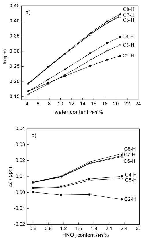
Figure 4. Chemical shift of \text{C}_2\text{mim}^+ protons in series II (a), and the relative chemical shift ( \Delta\delta ) of \text{C}_2\text{mim}^+ protons between series I and series I' ( \Delta\delta = \delta_{\text{Series I}} - \delta_{\text{Series I}'} ) (b).
