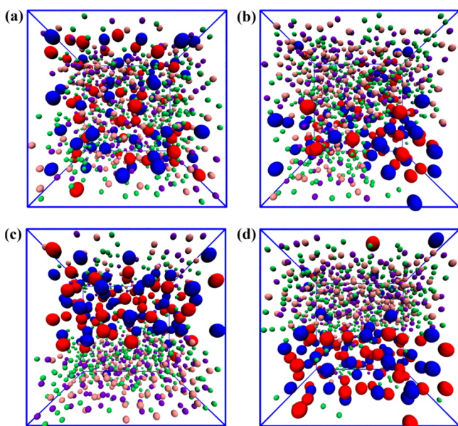
Figure 5. Simulation of the phase separation in the S-138. (a–d) Snapshots at 0, 100, 200, and 300 ns, respectively, which are exhibited by VMD 30 software package at drawing method “Beads”: blue beads represent C_2mim^+ , red beads represent NTf_2^- , violet beads represent H_3O^+ , pink beads represent NO_3^- , and lime beads represent water molecules.
