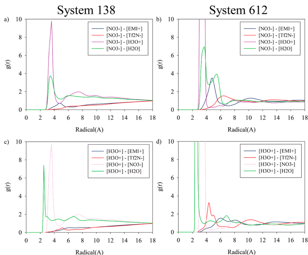
Figure 9. Radical distribution function (RDF) of different molecules around the nitric acid in S-138 (a,c) and S-612 (b,d), respectively.
