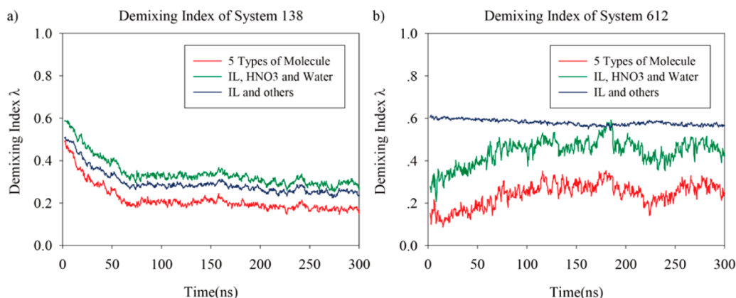
Figure 6. Demixing index \lambda in (a) S-138 and (b) S-612 as a function of time (averaged every 0.5 ns).
